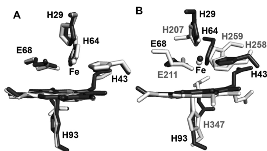
Figure 4. Overlay of Fe II -ZnPPFeMb1 (PDB ID: 4MXK, dark gray) with Fe II -FeMb1 (PDB ID: 3K9Z, light gray) (A), and cNOR (PDB ID: 3OOR, light gray) (B). Figures were generated using PyMol.
