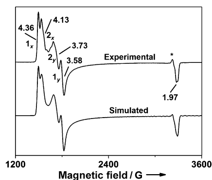
Figure 5. X-band EPR spectrum of a sample containing 0.7 mM ZnPPFeMb1 in the presence of 1.0 equiv FeCl 2 and 20 equiv of NO in 50 mM Bis-Tris buffer pH 7.3, and the simulated spectrum. Excess NO was used to ensure saturation of the Fe B site. Experimental parameters: T = 5 K, microwave frequency = 9.053 GHz, microwave power = 20 dB, modulation amplitude = 4 G. g values and the components are labeled. *A radical-type peak (< 1 %).
